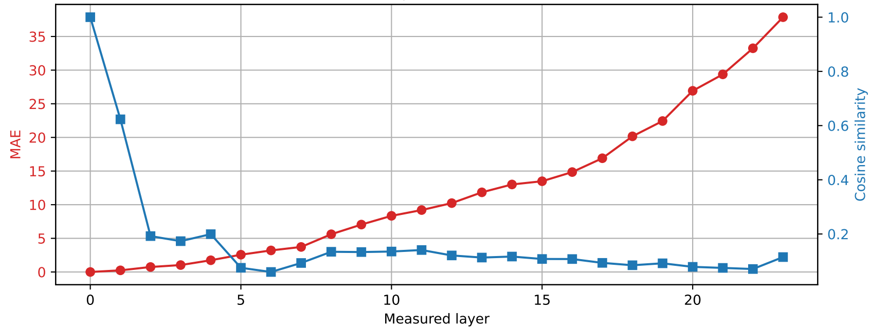
SmolLM2-1.7B-Instruct | Prompt 1 Spared layer 9 | Hybrid vs unquantized
