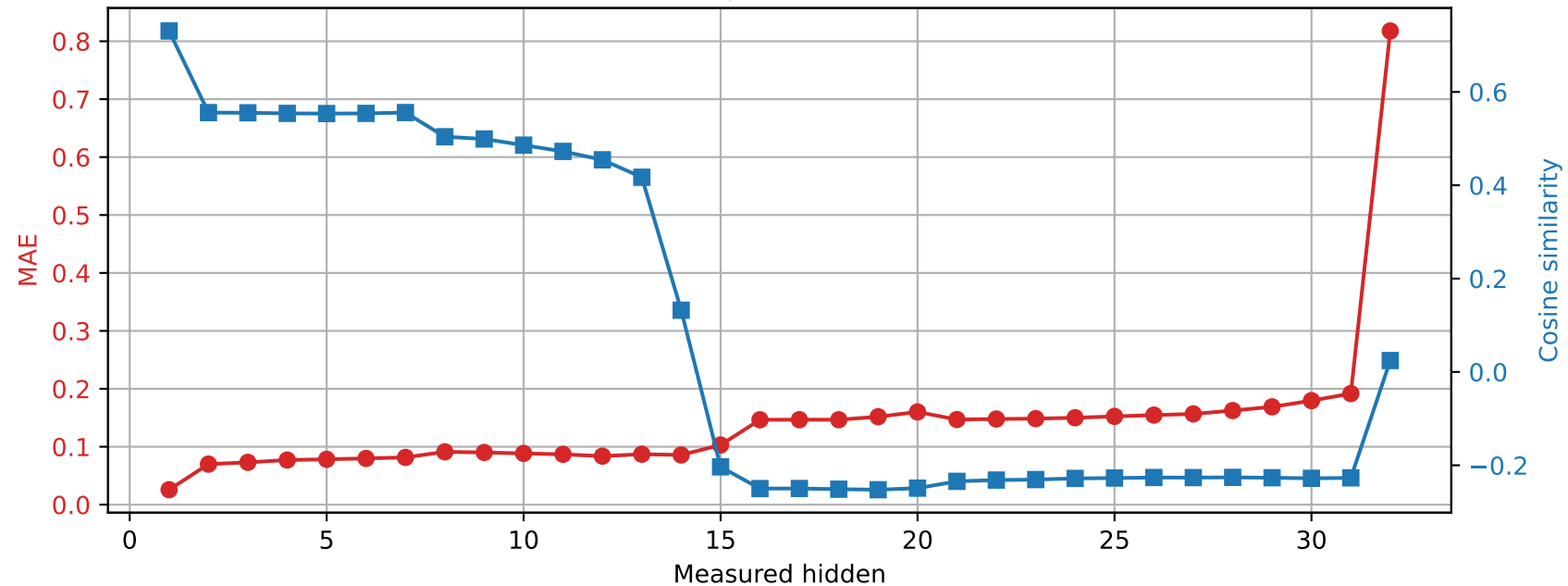
OLMo-7B-hf | Prompt 1 Spared layer 12 | Unquantized vs hybrid
