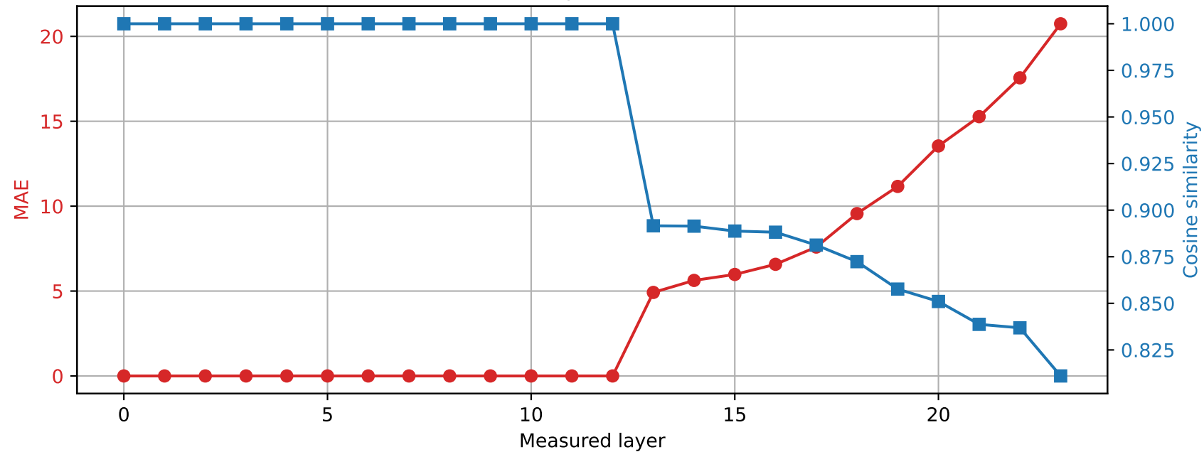
SmolLM2-1.7B-Instruct | Prompt 1 Spared layer 12 | Hybrid vs quantized
