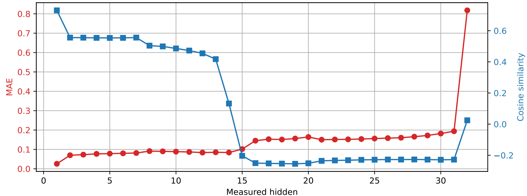
OLMo-7B-hf | Prompt 1 Spared layer 16 | Unquantized vs hybrid
