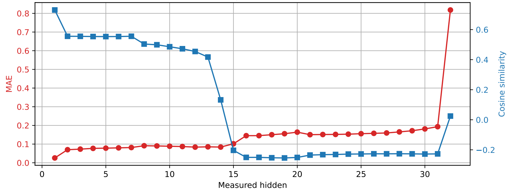
OLMo-7B-hf | Prompt 1 Spared layer 17 | Unquantized vs hybrid
