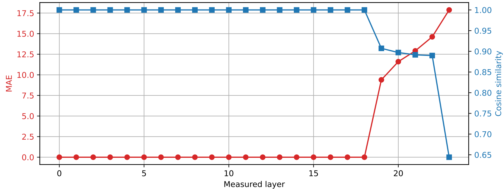
SmolLM2-1.7B-Instruct | Prompt 1 Spared layer 18 | Hybrid vs quantized
