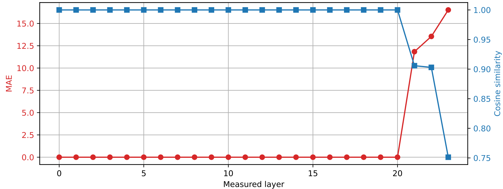
SmolLM2-1.7B-Instruct | Prompt 1 Spared layer 20 | Hybrid vs quantized
