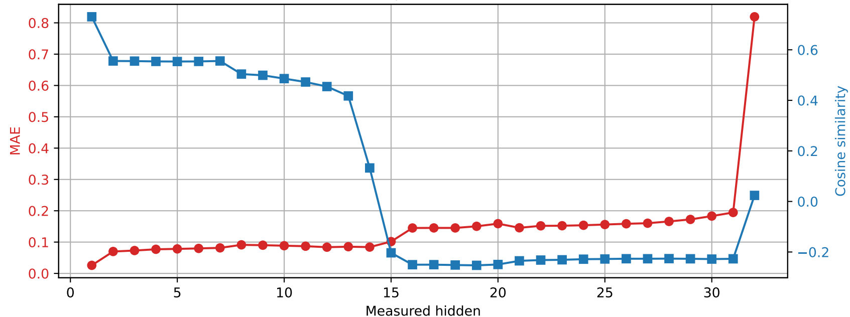
OLMo-7B-hf | Prompt 1 Spared layer 21 | Unquantized vs hybrid
