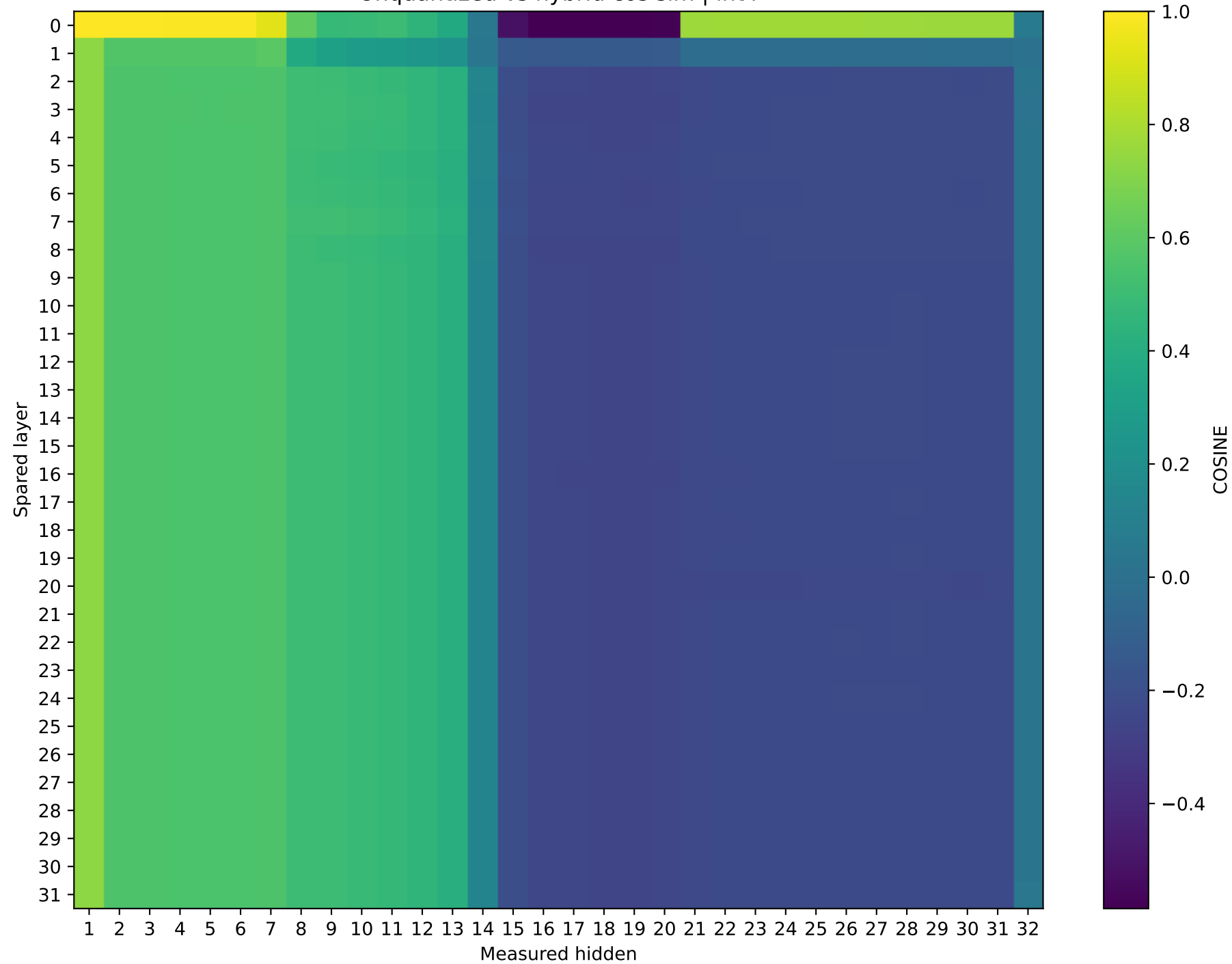
OLMo-7B-hf | Prompt 1 Unquantized vs hybrid cos sim | int4
