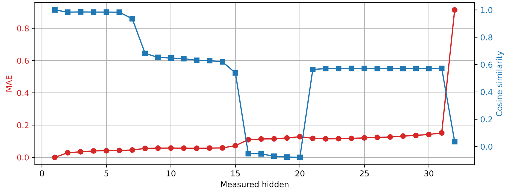
OLMo-7B-hf | Prompt 2 Spared layer 0 | Unquantized vs hybrid
