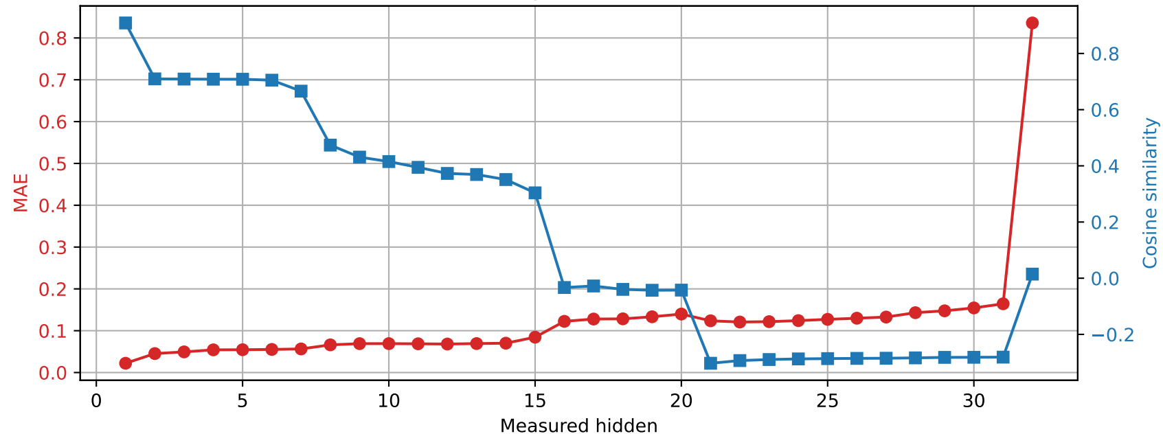
OLMo-7B-hf | Prompt 2 Spared layer 3 | Unquantized vs hybrid
