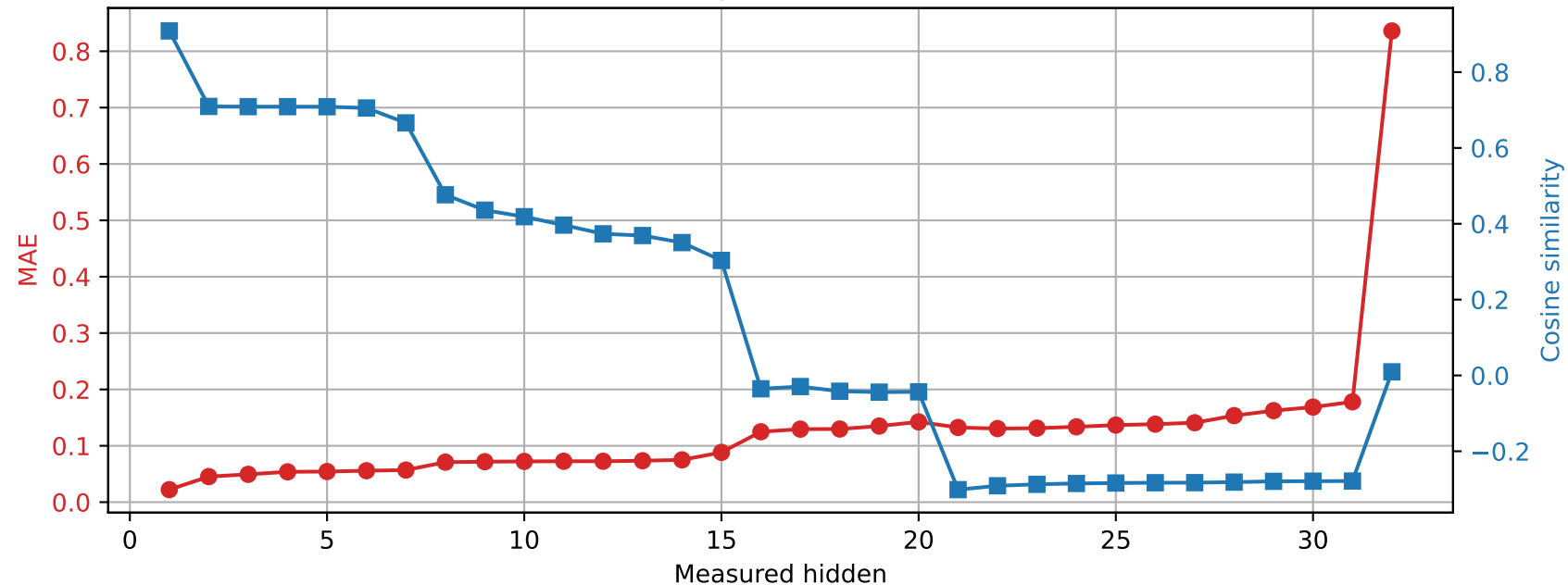
OLMo-7B-hf | Prompt 2 Spared layer 7 | Unquantized vs hybrid
