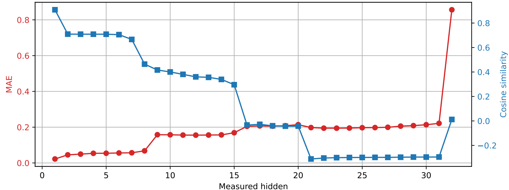
OLMo-7B-hf | Prompt 2 Spared layer 8 | Unquantized vs hybrid
