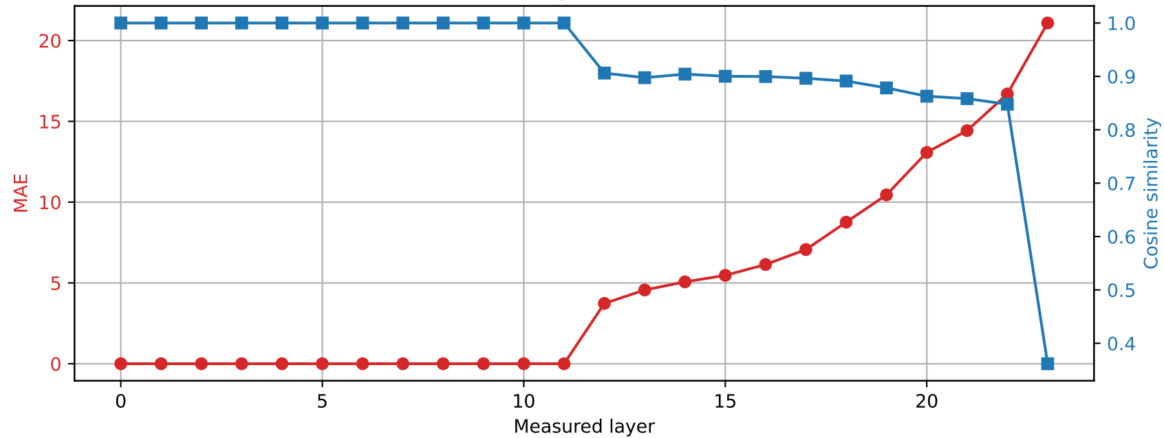
SmolLM2-1.7B-Instruct | Prompt 2 Spared layer 11 | Hybrid vs quantized
