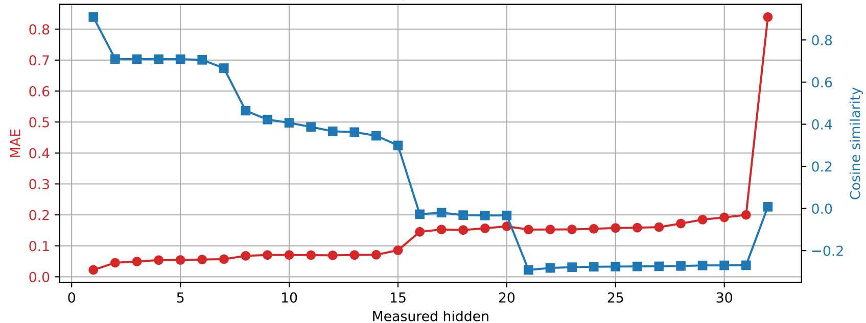
OLMo-7B-hf | Prompt 2 Spared layer 15 | Unquantized vs hybrid
