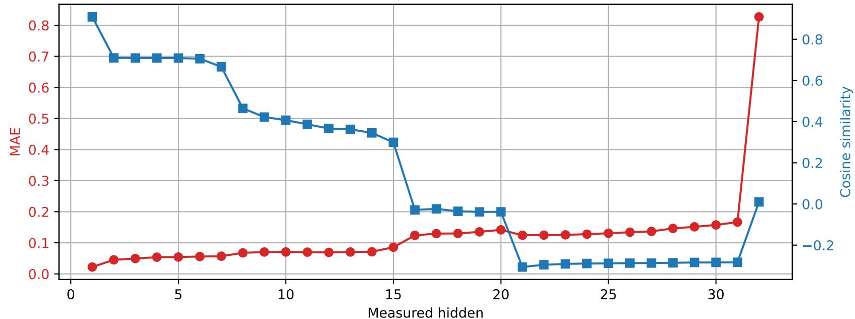
OLMo-7B-hf | Prompt 2 Spared layer 21 | Unquantized vs hybrid
