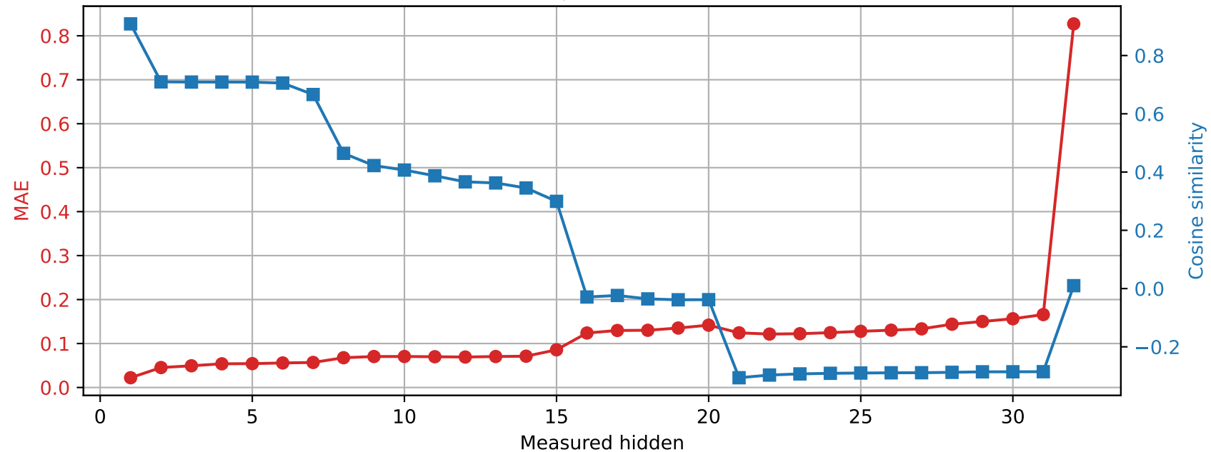
OLMo-7B-hf | Prompt 2 Spared layer 25 | Unquantized vs hybrid
