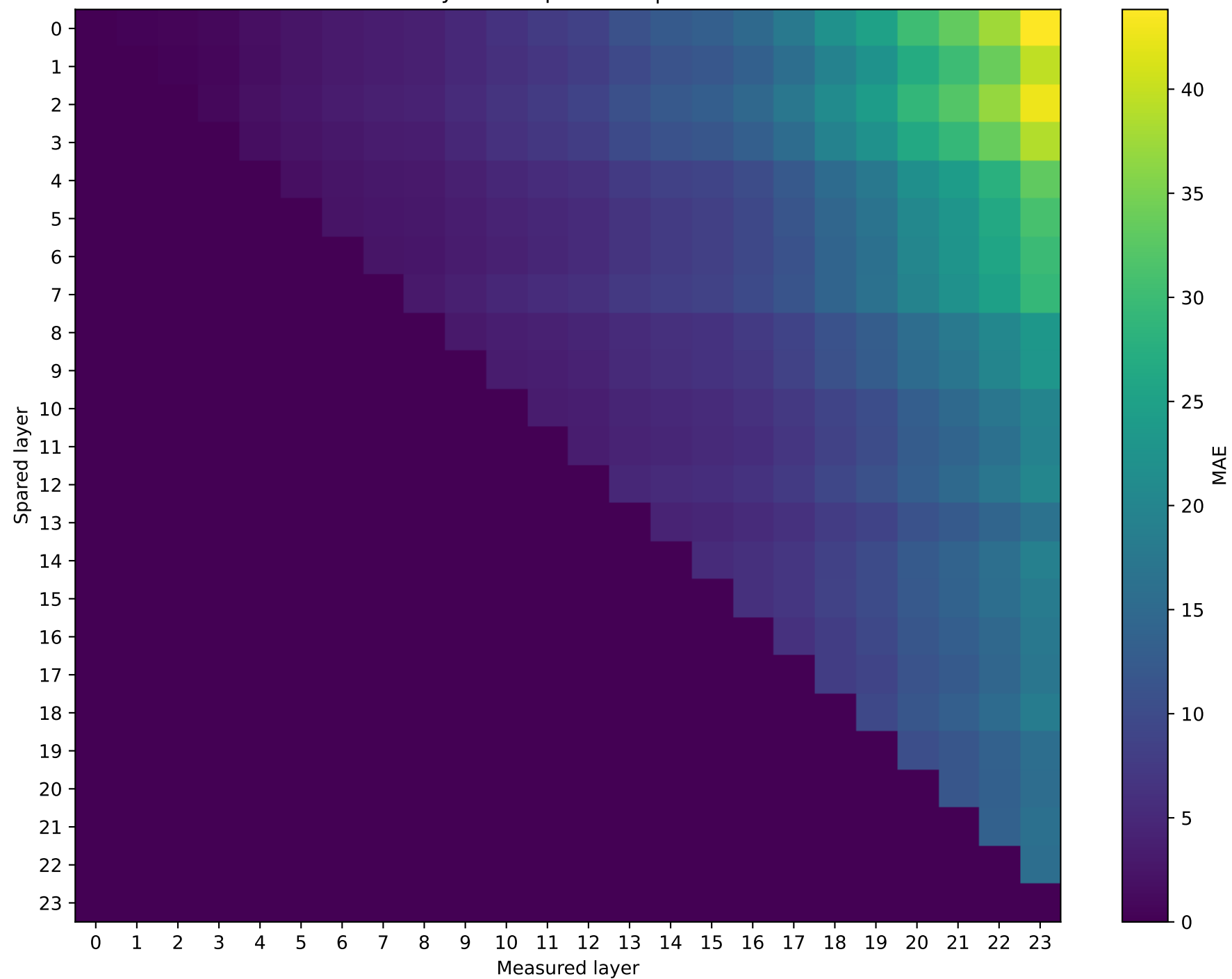
SmolLM2-1.7B-Instruct | Prompt 3 Hybrid vs quantized | int4
