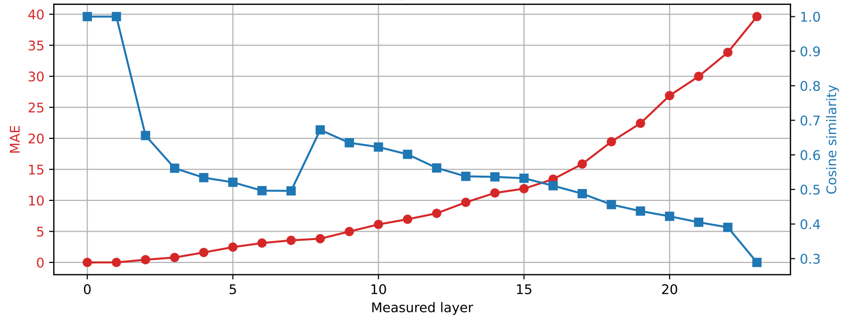
SmolLM2-1.7B-Instruct | Prompt 3 Spared layer 1 | Hybrid vs quantized
