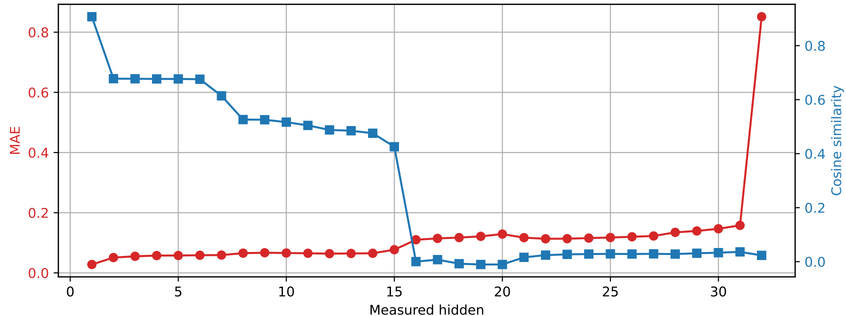
OLMo-7B-hf | Prompt 3 Spared layer 2 | Unquantized vs hybrid
