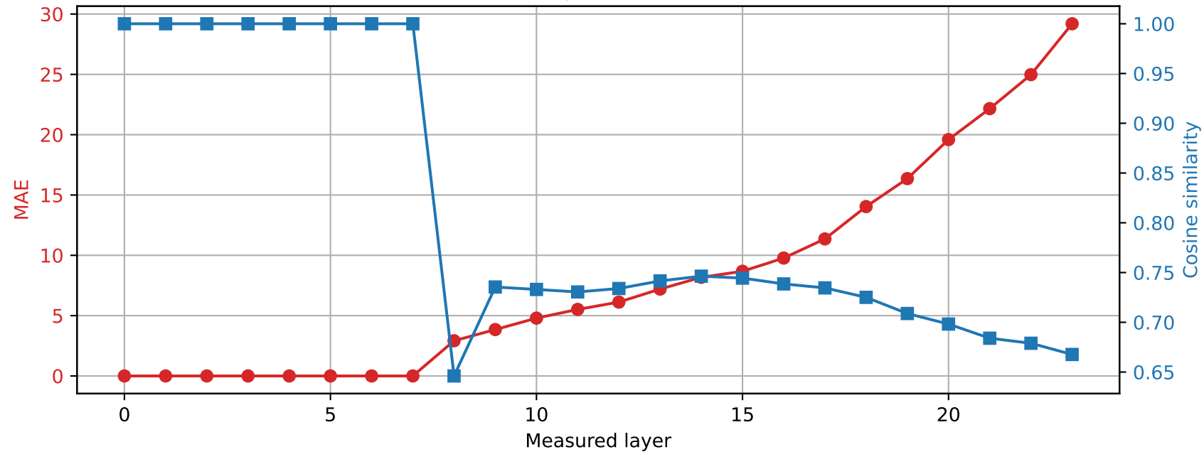
SmolLM2-1.7B-Instruct | Prompt 3 Spared layer 7 | Hybrid vs quantized
