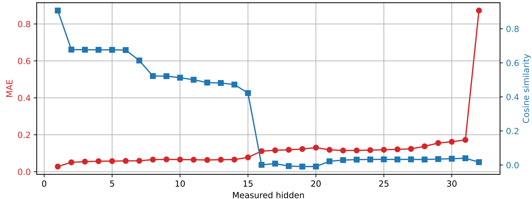
OLMo-7B-hf | Prompt 3 Spared layer 12 | Unquantized vs hybrid
