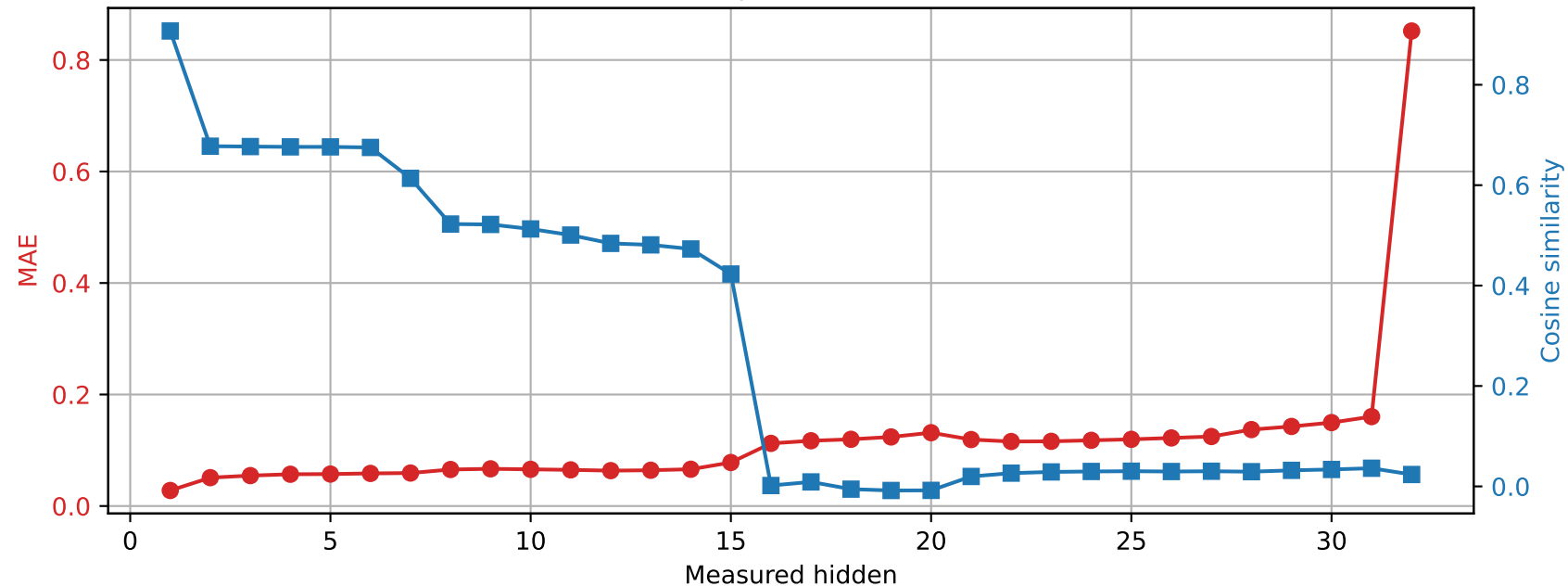
OLMo-7B-hf | Prompt 3 Spared layer 13 | Unquantized vs hybrid
