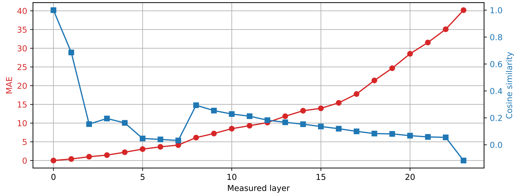
SmolLM2-1.7B-Instruct | Prompt 3 Spared layer 18 | Hybrid vs unquantized
