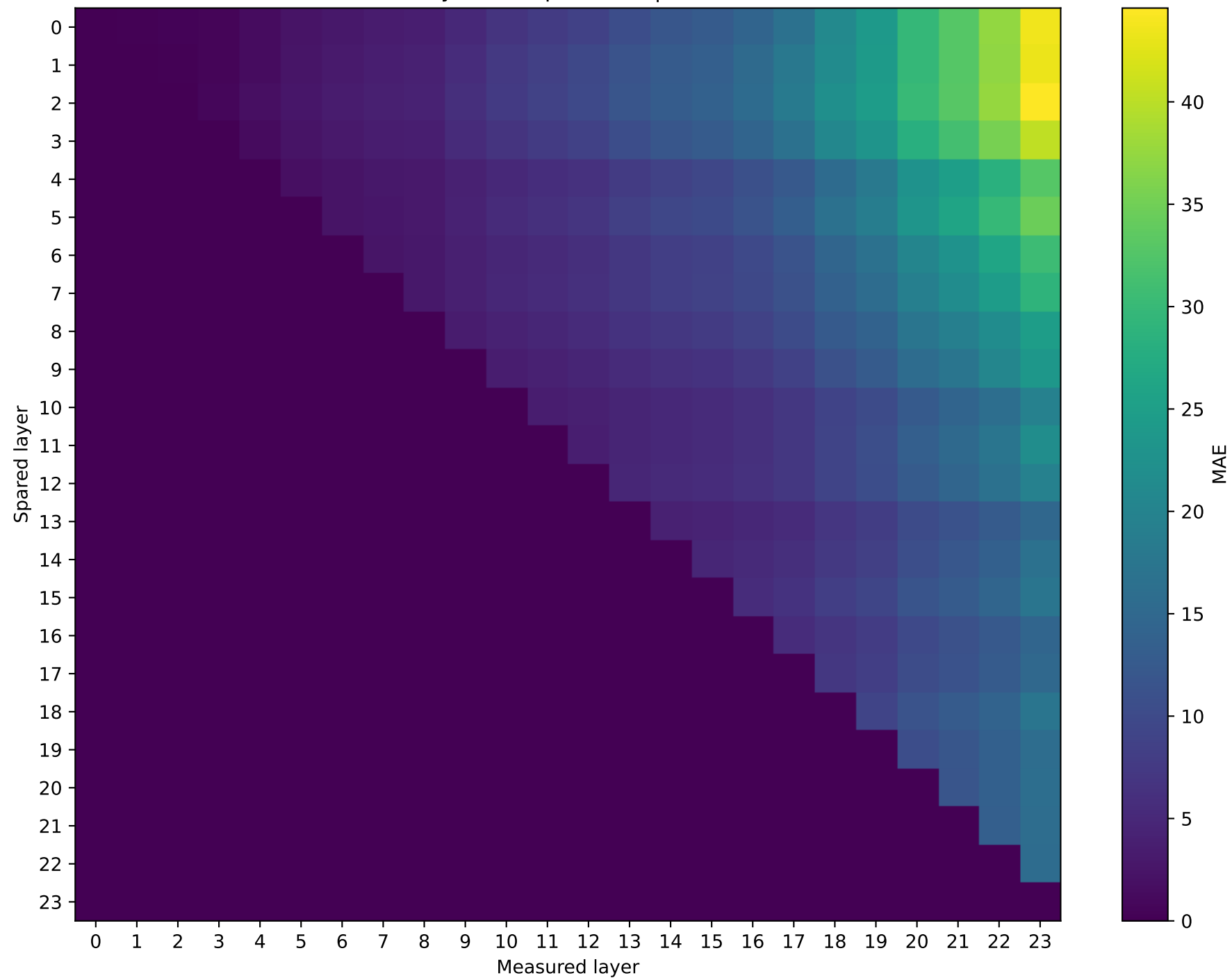
SmolLM2-1.7B-Instruct | Prompt 4 Hybrid vs quantized | int4
