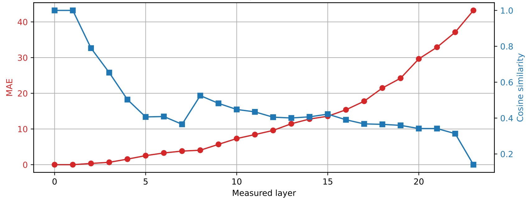
SmolLM2-1.7B-Instruct | Prompt 4 Spared layer 1 | Hybrid vs quantized
