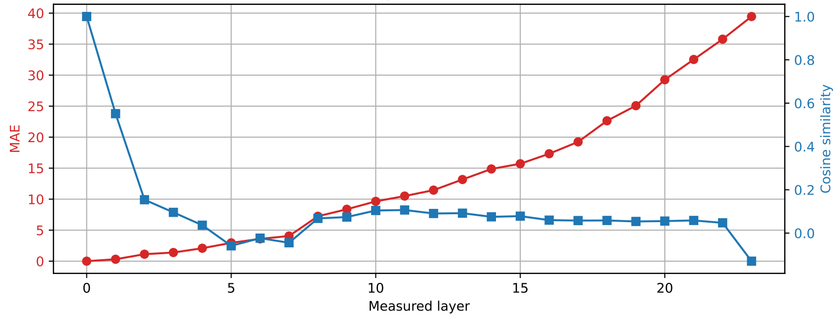
SmolLM2-1.7B-Instruct | Prompt 4 Spared layer 1 | Hybrid vs unquantized
