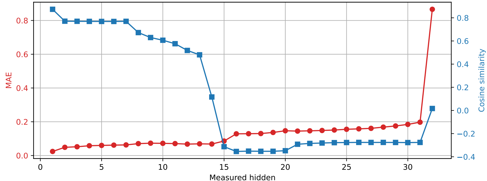
OLMo-7B-hf | Prompt 4 Spared layer 3 | Unquantized vs hybrid
