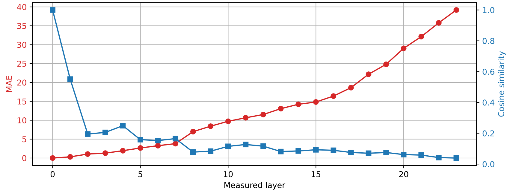
SmolLM2-1.7B-Instruct | Prompt 4 Spared layer 3 | Hybrid vs unquantized
