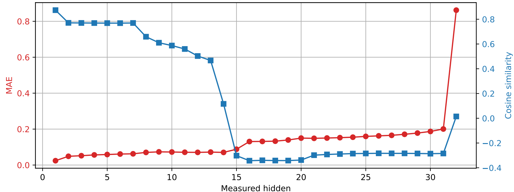
OLMo-7B-hf | Prompt 4 Spared layer 11 | Unquantized vs hybrid
