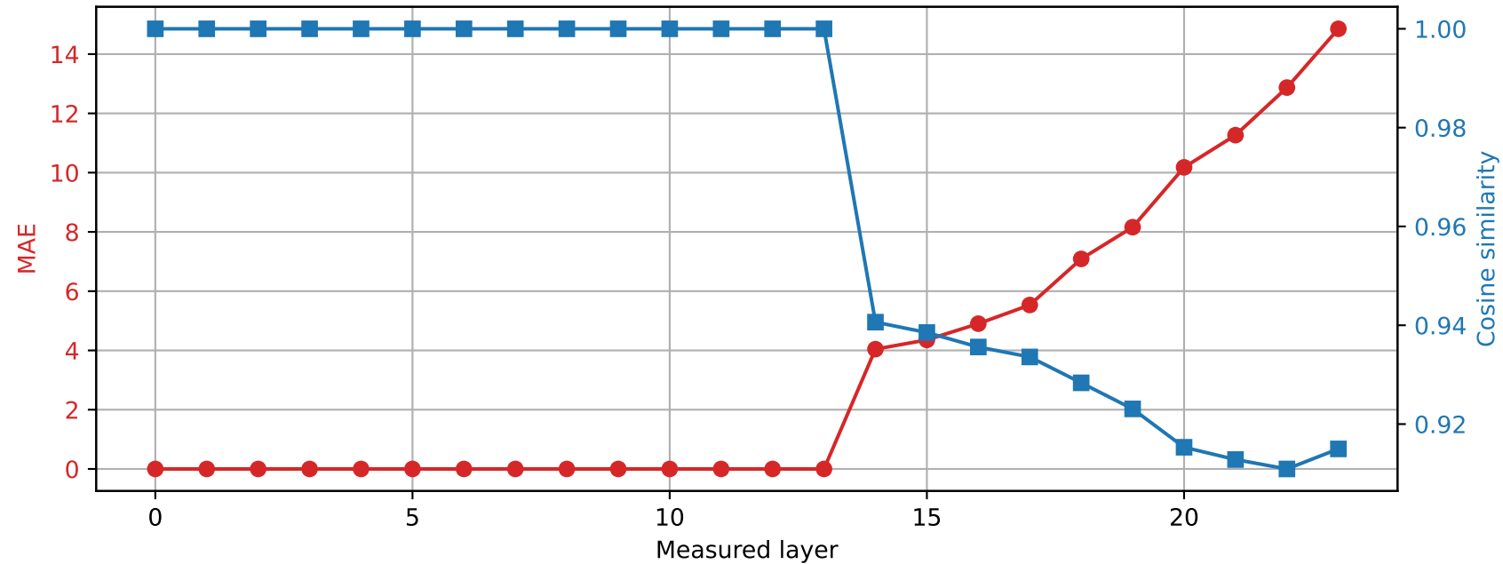
SmolLM2-1.7B-Instruct | Prompt 4 Spared layer 13 | Hybrid vs quantized
