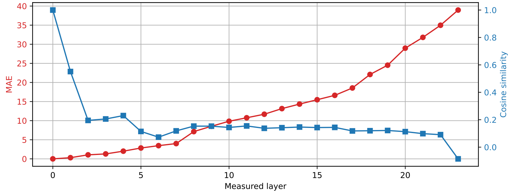
SmolLM2-1.7B-Instruct | Prompt 4 Spared layer 14 | Hybrid vs unquantized
