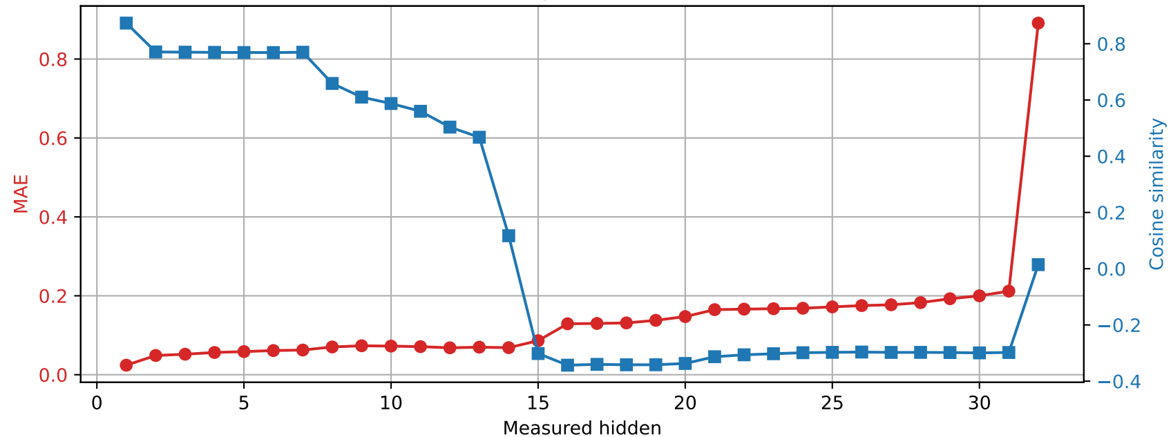
OLMo-7B-hf | Prompt 4 Spared layer 20 | Unquantized vs hybrid
