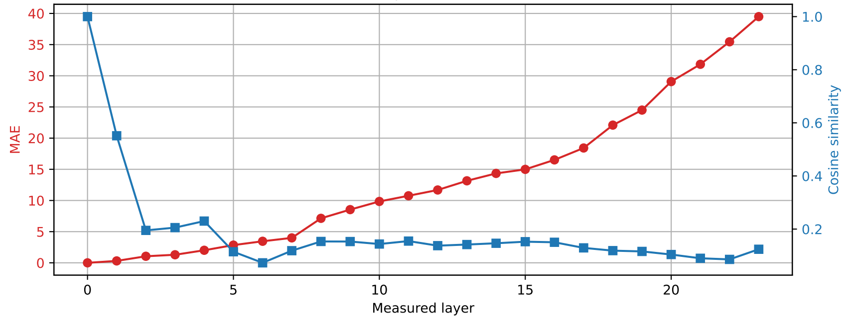
SmolLM2-1.7B-Instruct | Prompt 4 Spared layer 22 | Hybrid vs unquantized
