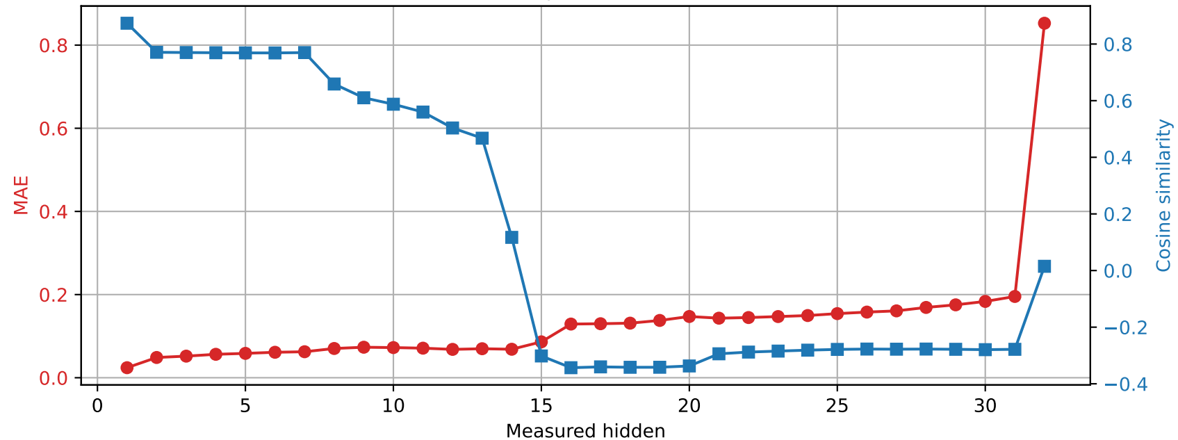
OLMo-7B-hf | Prompt 4 Spared layer 24 | Unquantized vs hybrid
