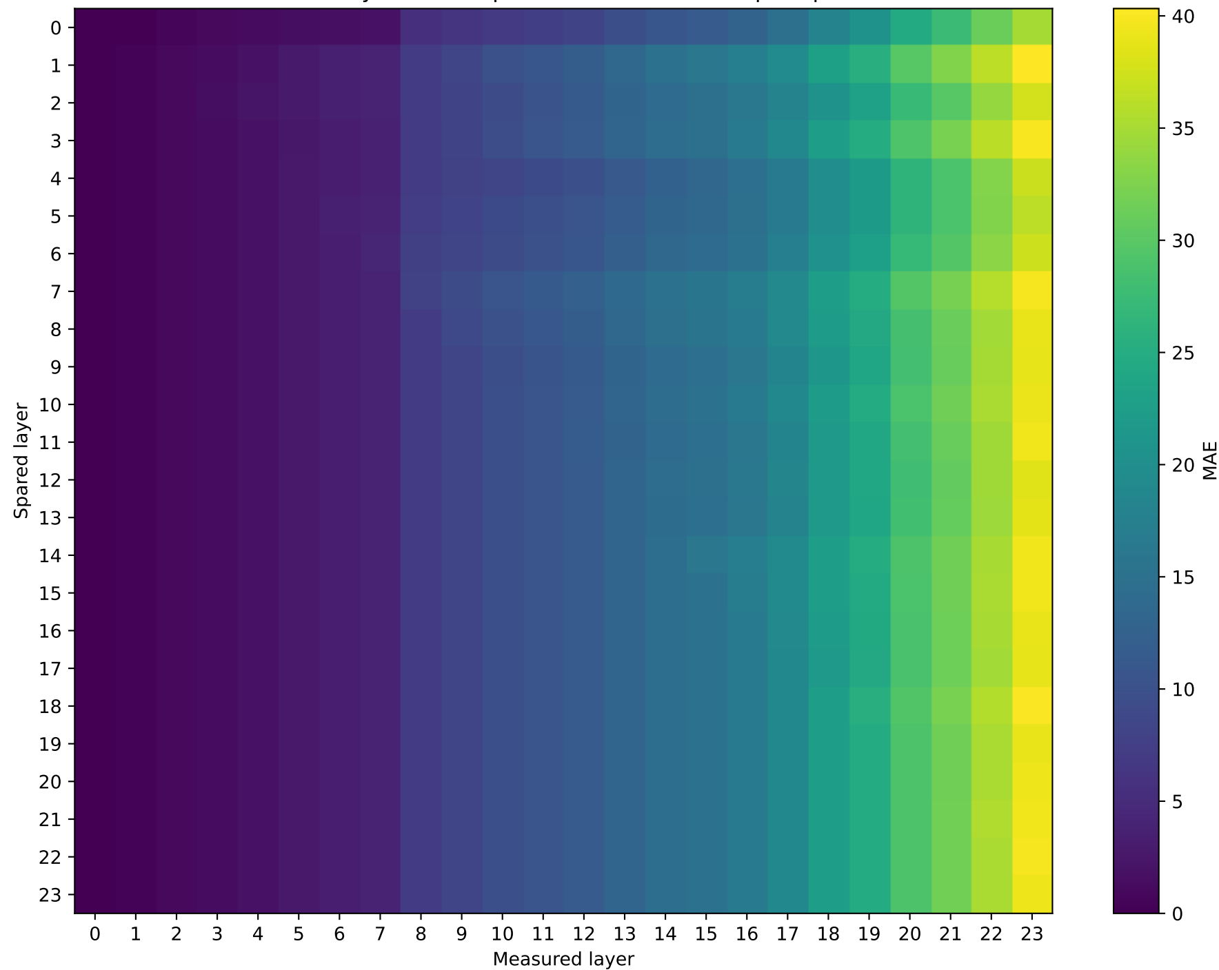
SmolLM2-1.7B-Instruct Mean hybrid vs unquantized MAE across 5 prompts
