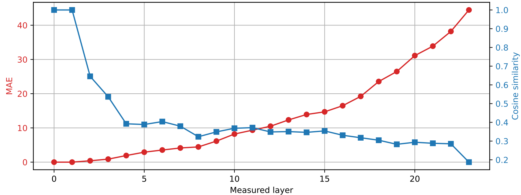
SmolLM2-1.7B-Instruct | Prompt 0 Spared layer 1 | Hybrid vs quantized
