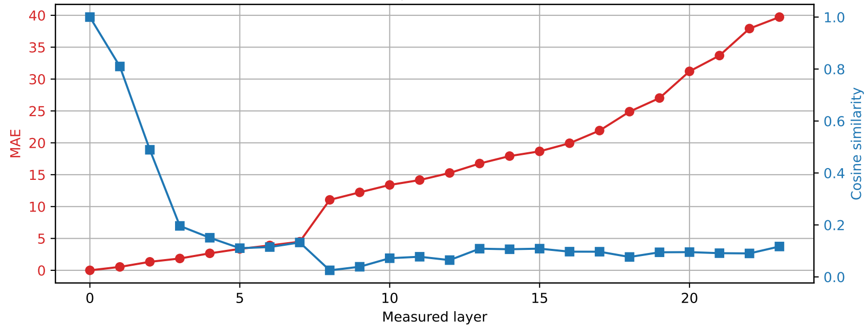
SmolLM2-1.7B-Instruct | Prompt 0 Spared layer 2 | Hybrid vs unquantized
