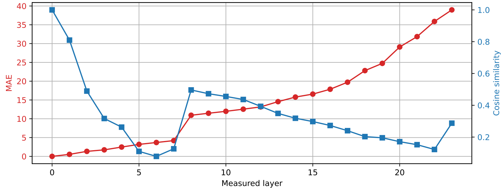
SmolLM2-1.7B-Instruct | Prompt 0 Spared layer 4 | Hybrid vs unquantized
