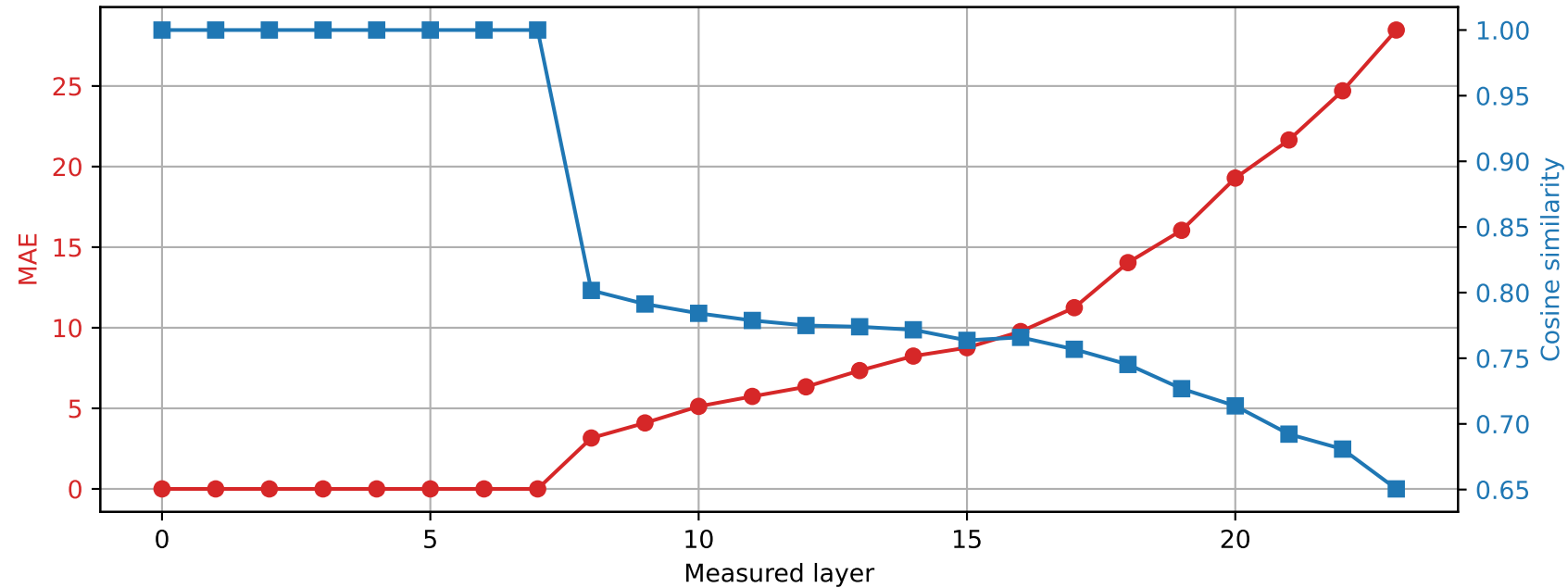
SmolLM2-1.7B-Instruct | Prompt 0 Spared layer 7 | Hybrid vs quantized
