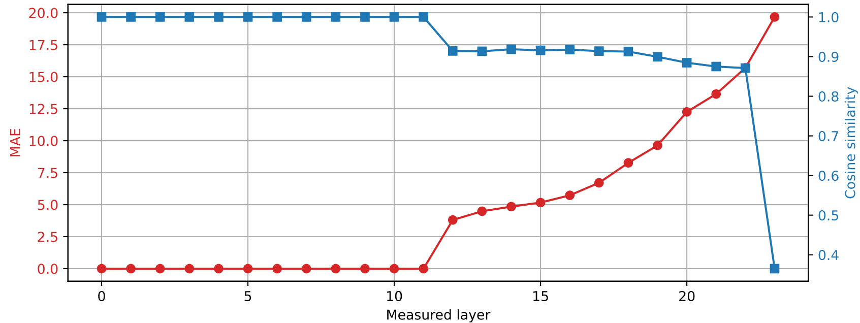
SmolLM2-1.7B-Instruct | Prompt 0 Spared layer 11 | Hybrid vs quantized
