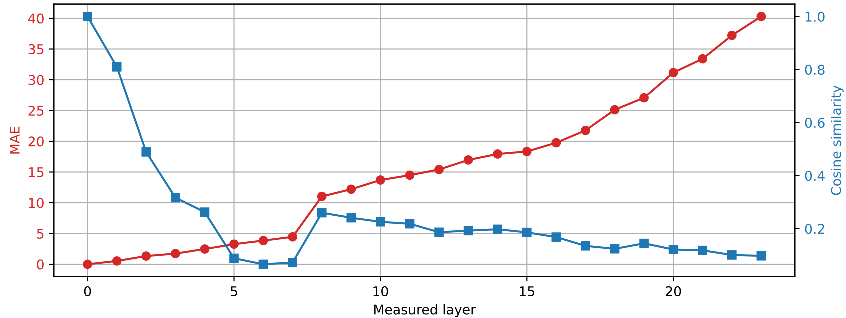
SmolLM2-1.7B-Instruct | Prompt 0 Spared layer 13 | Hybrid vs unquantized
