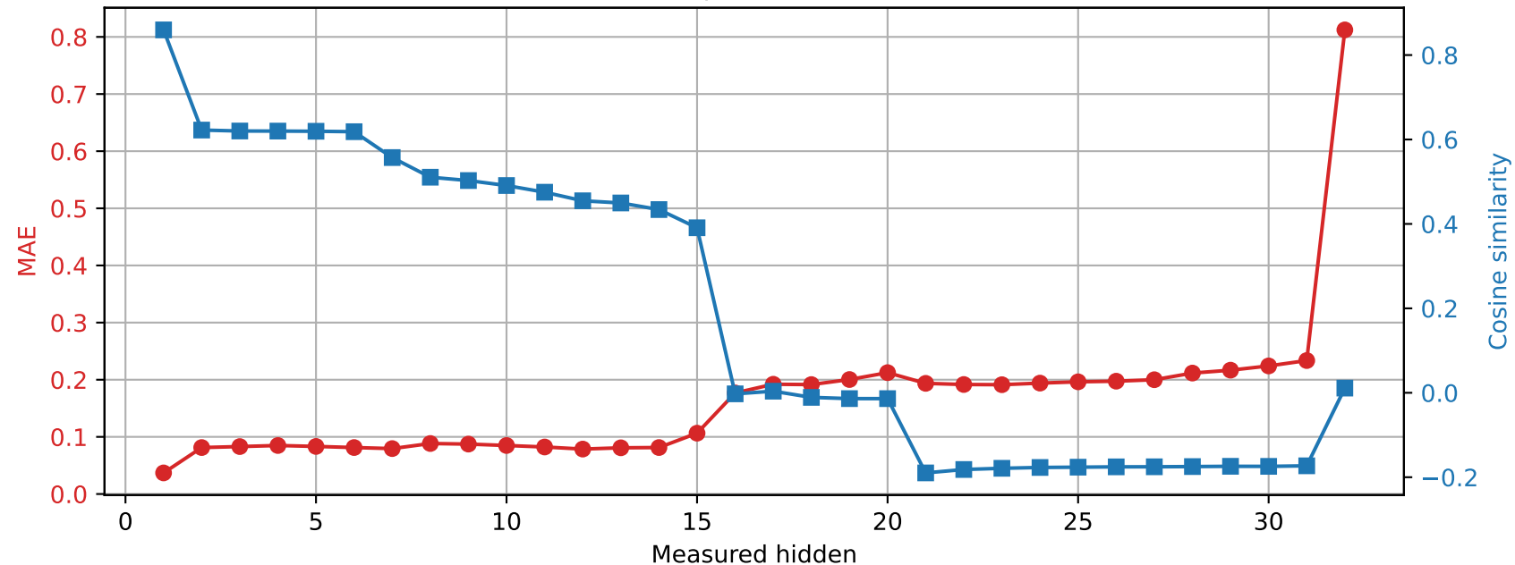
OLMo-7B-hf | Prompt 0 Spared layer 16 | Unquantized vs hybrid
