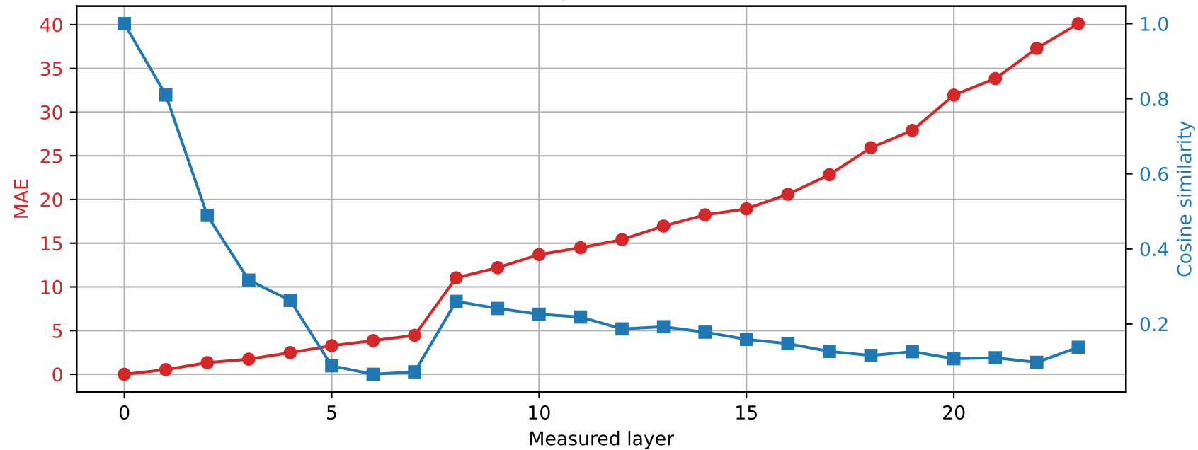
SmolLM2-1.7B-Instruct | Prompt 0 Spared layer 16 | Hybrid vs unquantized
