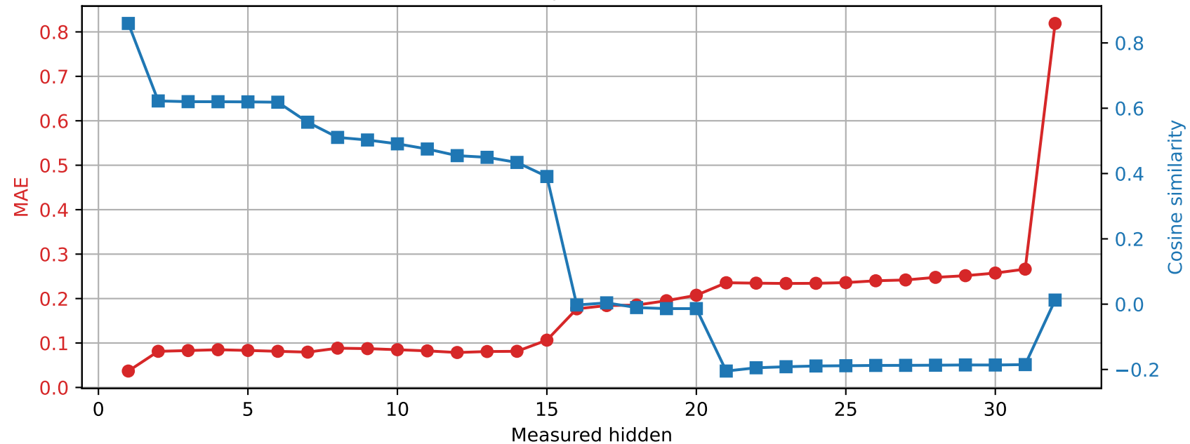
OLMo-7B-hf | Prompt 0 Spared layer 20 | Unquantized vs hybrid
