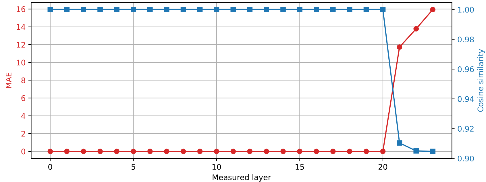
SmolLM2-1.7B-Instruct | Prompt 0 Spared layer 20 | Hybrid vs quantized
