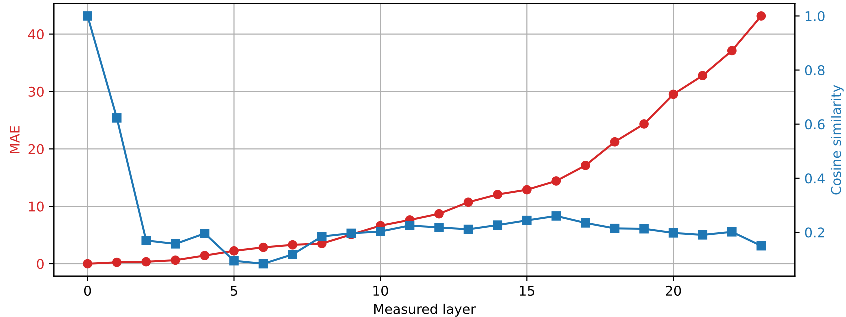
SmolLM2-1.7B-Instruct | Prompt 1 Spared layer 0 | Hybrid vs quantized
