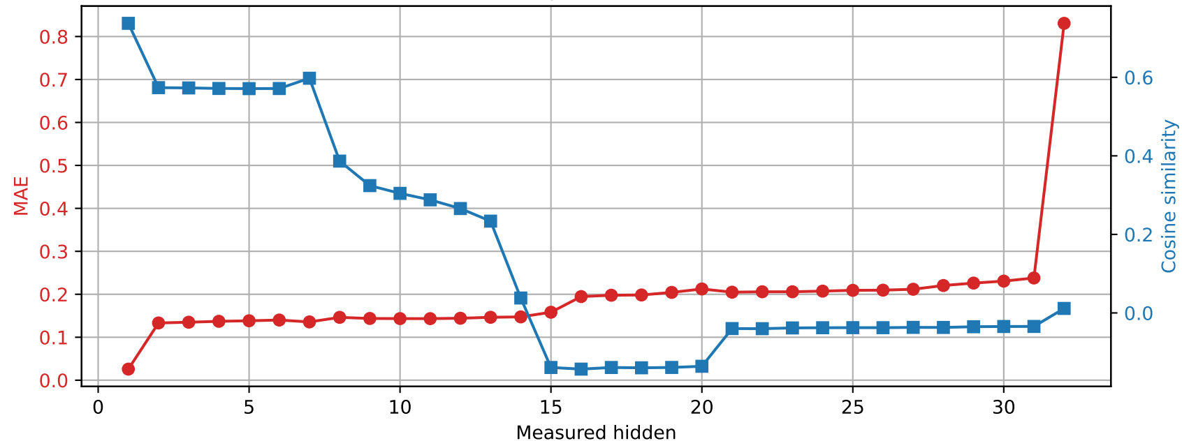
OLMo-7B-hf | Prompt 1 Spared layer 1 | Unquantized vs hybrid
