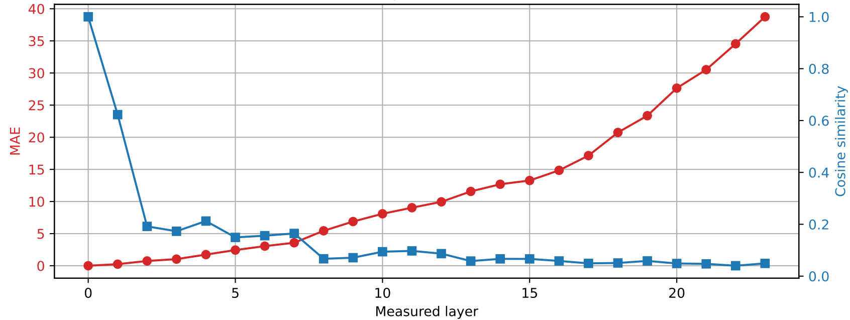
SmolLM2-1.7B-Instruct | Prompt 1 Spared layer 3 | Hybrid vs unquantized
