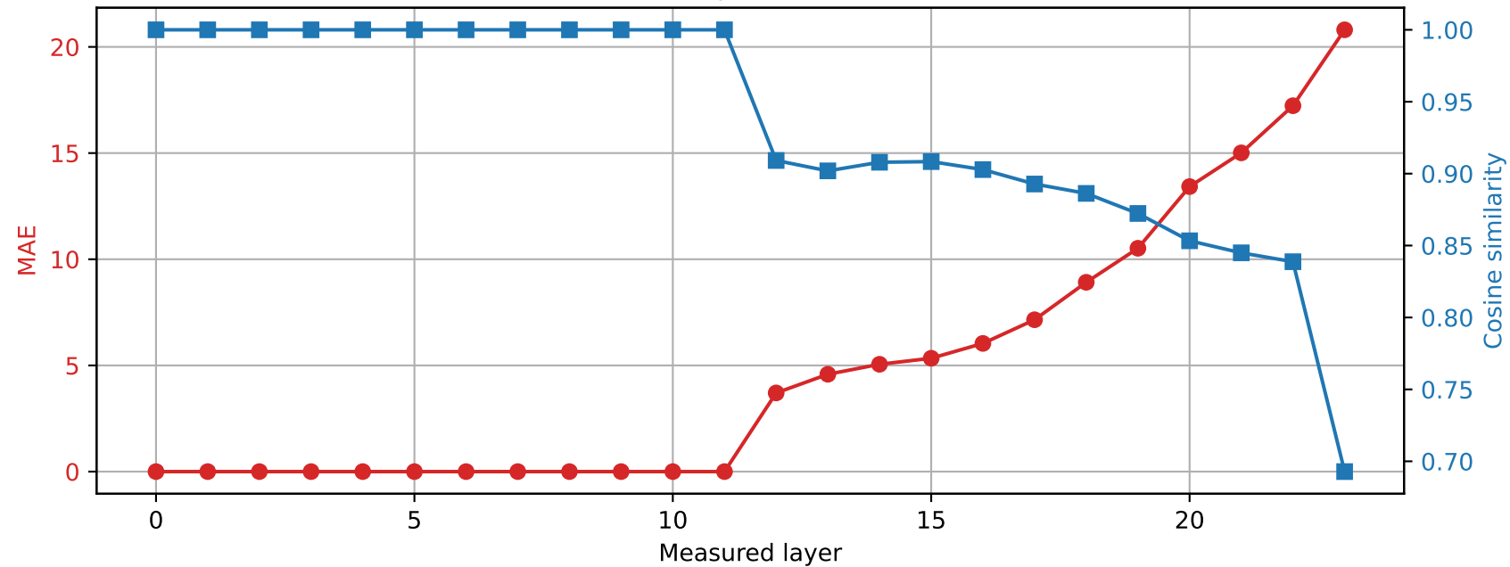
SmolLM2-1.7B-Instruct | Prompt 1 Spared layer 11 | Hybrid vs quantized
